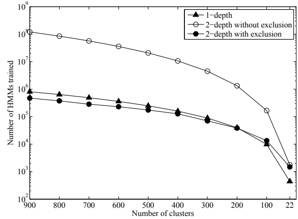
Fig. 5. Computational comparison
