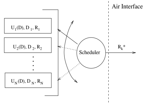
Fig. 1. System Model with N packets.
