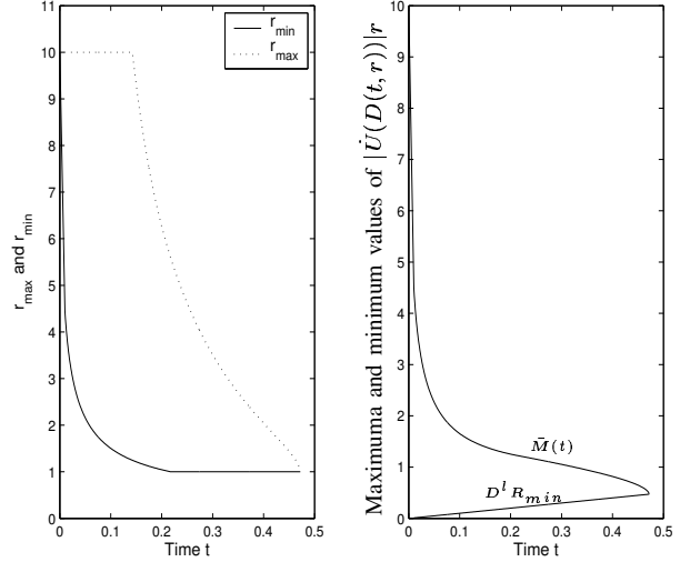
Fig. 8. (a) Range of active rates from r_{min} to r_{max} ; (b) Decision metric envelope \bar{M}(t) vs. t .
