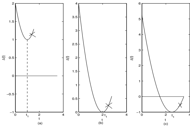
Fig. 10. Example trajectories of \Delta(t) vs. t with \dot{\Delta}(t_1) = 0 : (a) shows \Delta(t_1) > 0 ; (b) shows \Delta(t_1) = 0 ; and (c) shows \Delta(t_1) < 0 ; Both cases (a) and (b) result in contradictions and so can not occur. Case (b) may only occur if t_1 = t_2^{out} .
