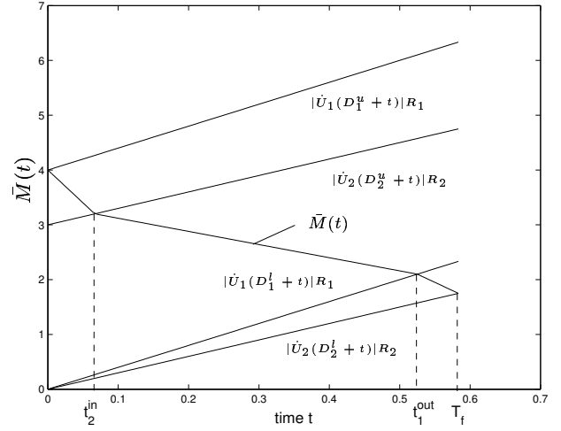
Fig. 2. An example of the time evolution of \bar{M}(t) , |\dot{U}_i(D_i^u + t)|R_i , and |\dot{U}_i(D_i^l + t)|R_i for a two-class system. The intersections of \bar{M}(t) with the other curves correspond to the times t = 0, t_2^{in}, t_1^{out}, T_f .
