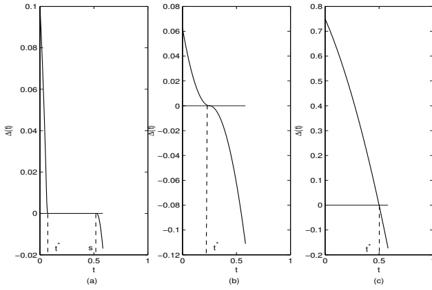
Fig. 9. Possible behaviors of \Delta(t) vs. t . (a) shows \Delta(t) = 0 and \dot{\Delta}(t) = 0 , for t \in (t^*, s) (a singular interval); (b) shows \Delta(t^*) = 0 and \dot{\Delta}(t^*) = 0 (no singular interval); and (c) shows \Delta(t^*) = 0 and \dot{\Delta}(t^*) < 0 (no singular interval).
