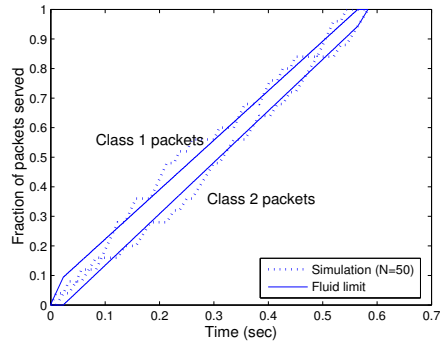
Fig. 5. The fraction of packets served over time with U(D) = -D^4 and uniform delays.
