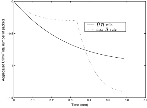
Fig. 7. The normalized aggregate utility over time for the Max R and UR rules.
