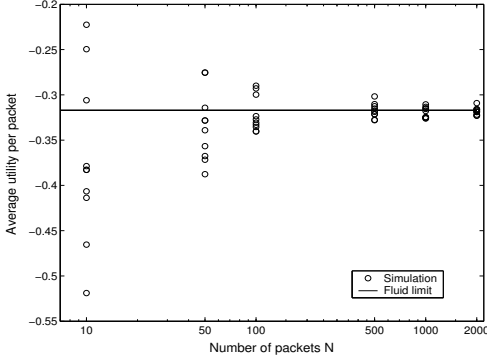
Fig. 6. The average utility per packet for different realizations of finite systems with N packets.
