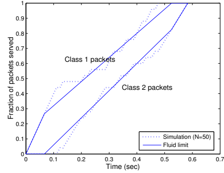
Fig. 4. Fraction of packets served over time with U(D) = -D^2 and uniform initial delays.
