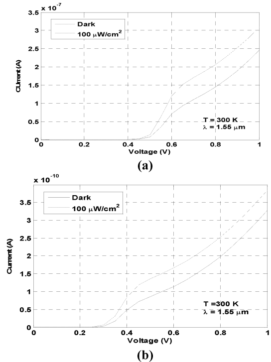
Figure 4 – Comparison of unpassivated (a) and passivated (b) devices at same voltages and optical powers.
