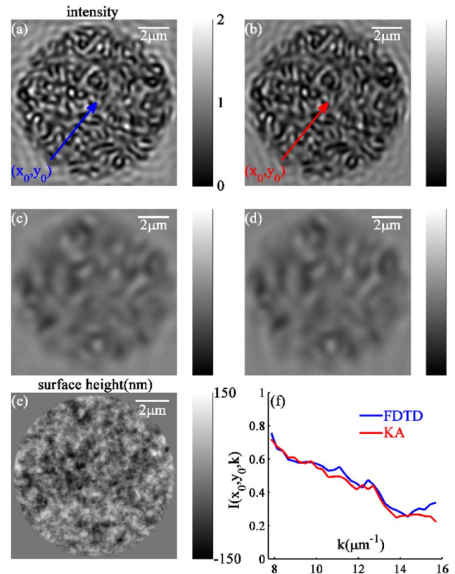
Fig. 2. Comparisons of (a), (c) FDTD-synthesized and (b), (d) KA-synthesized microscope images of a rough surface with \sigma_b = 35 nm and l_{c_b} = 170 nm: \lambda = 400 nm for (a) and (b); \lambda = 800 nm for (c) and (d). (e) Height map of the same surface. (f) Comparative FDTD- and KA-synthesized center pixel (x_0, y_0) spectra.
